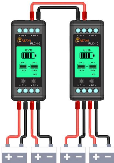
③ 4PCS Batteries Connect
